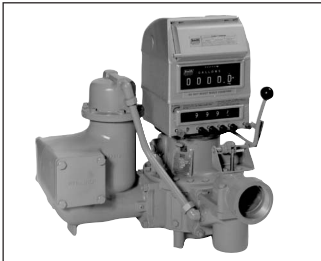
T20 Meter with T3A Air eliminator, SPG3 Faucet, Preset Counter, Counter, and Ticket Printer - Model T20-Z
